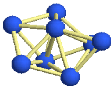
Fe8
