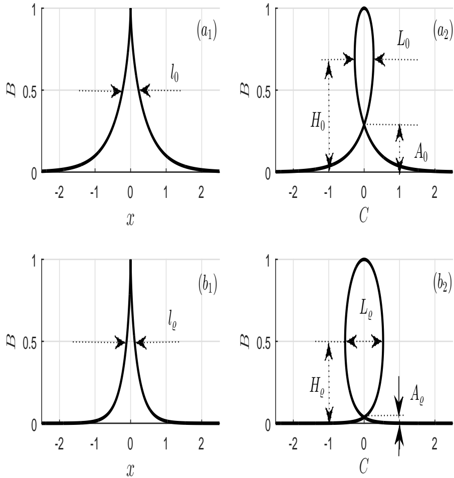
Figure 11: Propagation of one-soliton solution B to the system Eq.(3.94) for s = 0 , with the eigenvalue \eta = 1 , \rho = 0.0625 at times t = 0 , depicted versus x and versus C (panels (a 1 ), (a 2 )) and the one-soliton solution B to the KMM-system Eq.(3.86) versus versus x and versus C (panels (b 1 ), (b 2 )). The parameters l_0 and l_\rho stand for the width at half maximum height, L_0 and L_\rho stand for the maximum width of the loop solitons, H_0 and H_\rho represent the magnitude at which the width of the loops solitons are maximal and A_0 and A_\rho represent the magnitude at which the cross over occurs.
