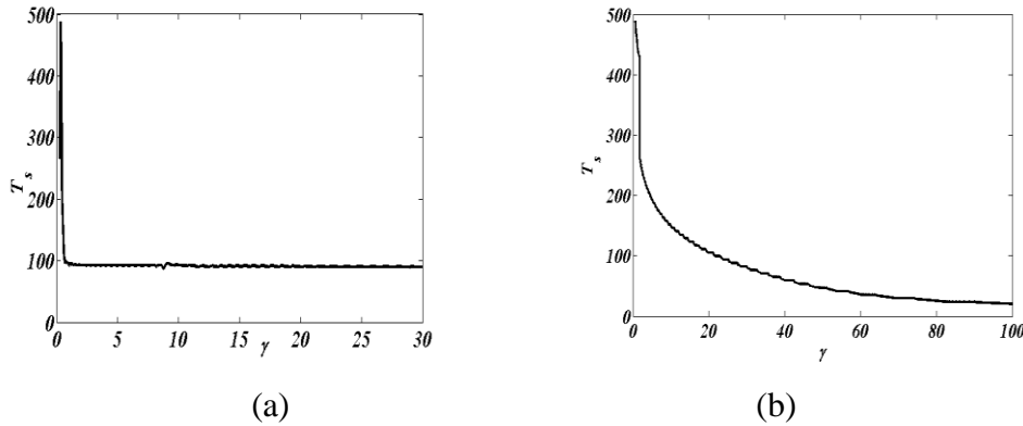
Figure 3.20 Synchronization time versus the adaptive control parameter \gamma : (a) for \mu=0.3 and (b) for \mu=5 .
