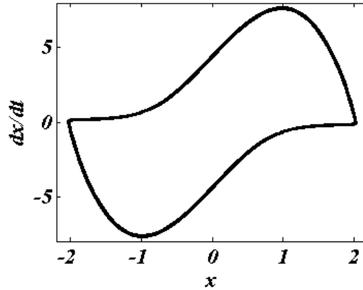
Figure 1.3: Phase portrait of the oscillator in the situation of \mu = 5 .
