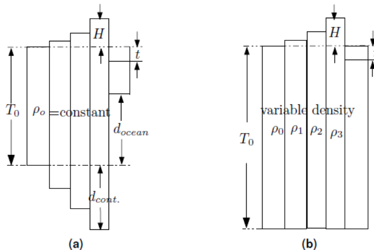
Figure 8: (a) Isostatic model of Airy; (b) Isostatic model of Pratt
