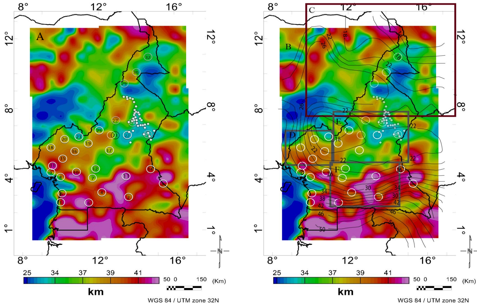
Figure 13: (A) Color code showing the crustal thicknesses or Moho depth of Cameroon and environs estimated from the World Gravity Map (WGM2012) data using two-dimensional (2D) radially-averaged power-spectrum analysis. The white circles with number in Fig.13 A and white circles in Fig. 13B represent the locations of the passive seismic station of Tokam et al. (2010) and Gallacher and Bastow (2012). (B) Color code showing the crustal thicknesses or Moho depth of Cameroon and environs estimated from the World Gravity Map (WGM2012) data using two-dimensional (2D) radially-averaged power-spectrum analysis. The box labeled “D”, “E” and “F” defines the sub-regions used by Nnange et al. (2000) to estimate the Moho depth using spectral analysis of ground gravity data. The solid black line with numbers represents the Moho depth estimates from Poudjom Djomani et al. (1995) using spectral analysis of ground gravity data. The red box labeled “B” defines the location of the sub-region used by Eyike and Ebbing (2015) to image the crustal thickness using gravity inversion.
