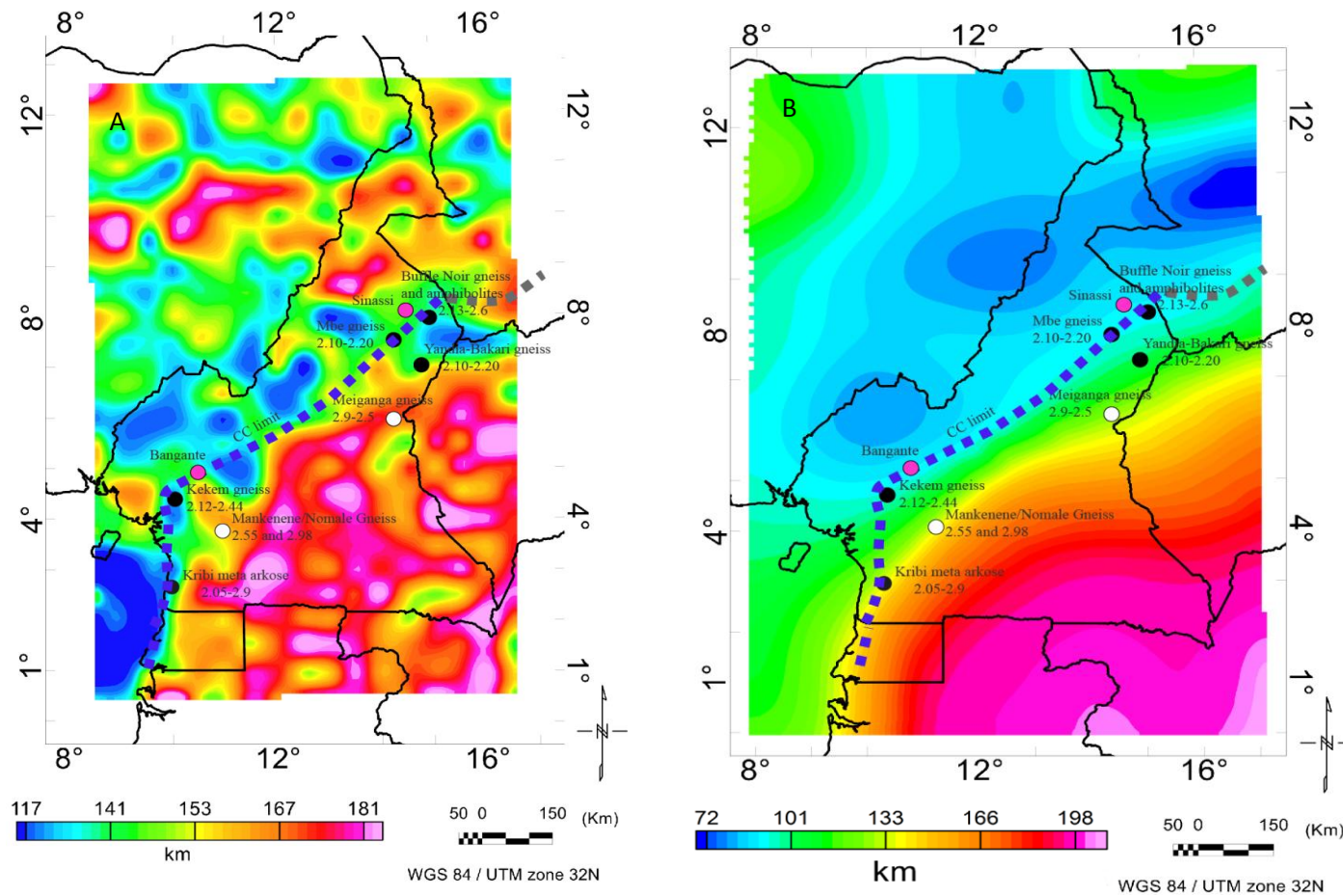
Figure 21: (A) Color-coded map showing lithosphere-asthenosphere (LAB)/Mid-lithosphere discontinuity (MLD) of Cameroon and its surrounding estimated from the World Gravity Map (WGM2012) data using two-dimensional (2D) radially-averaged power-spectrum analysis. CC = Congo craton. (B) Color code map showing Lithosphere - Asthenosphere Boundary (LAB) depth estimates for Cameroon and its surroundings obtained from the thermal inversion of seismic data. CC = Congo craton. The blue dash line represents the northwestern margin of the Congo craton (CC) and the grey dashed line the unconstrained CC limit. The black circle represents Palaeoproterozoic occurrences (Penaye et al. 2004). The white circle represents the Archaean occurrences (Tchakounte et al. 2017 and Ganwa et al. 2016). The Pink circle represents the localization of Sinassi and Bangante where geochemical evidence subduction environment has been found (Tchouankoue et al. , 2016; Bouyo et al. , 2015; 2016).
