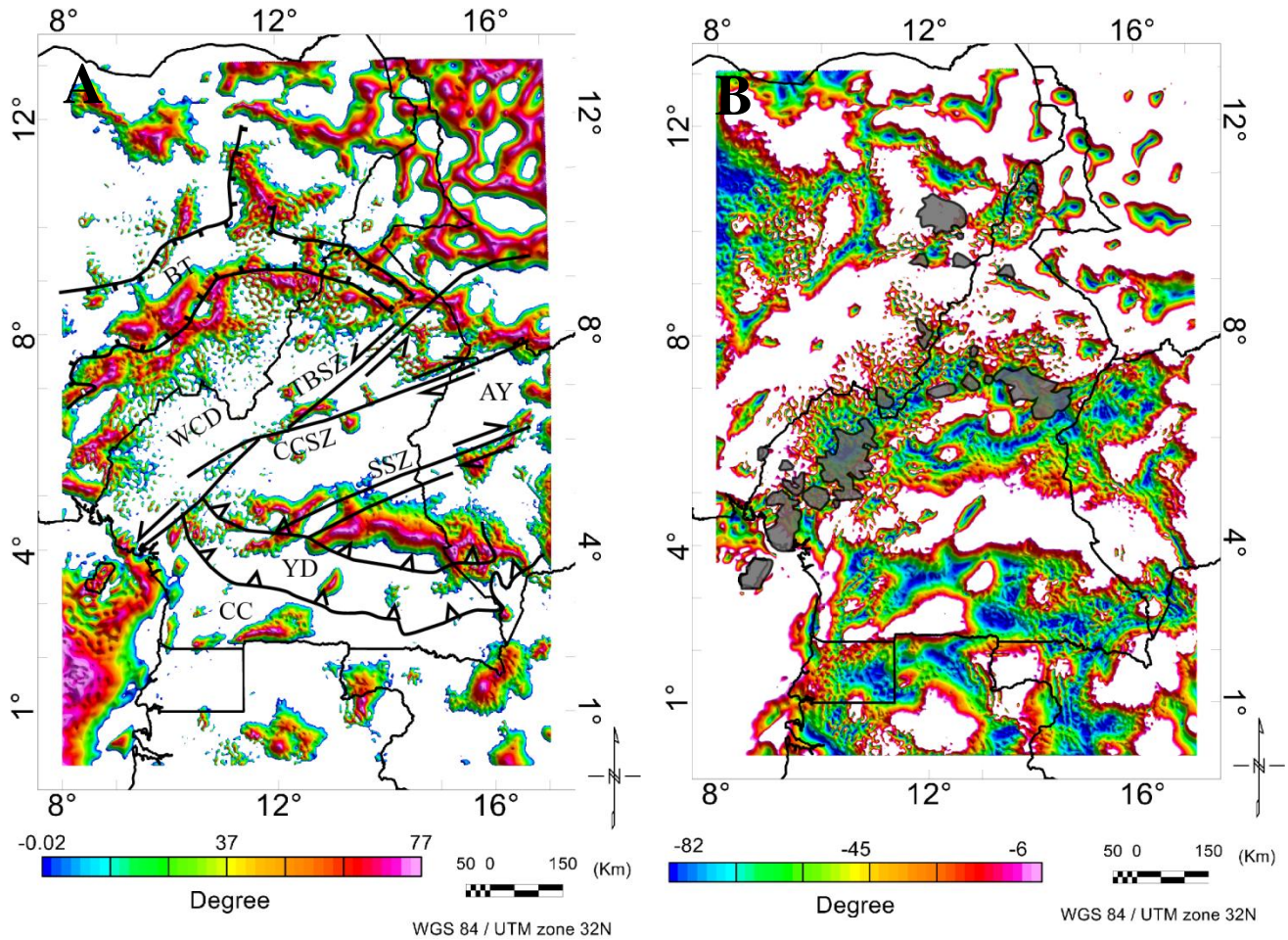
Figure 11: Positive (A) and negative (B) tilt derivative maps of southern Cameroon and surrounding regions extracted from the vertical tilt derivative of the 2 km upward continuation map shown in Fig. 10 A. CC= Congo craton, YD = Yaounde domain, AY = Adamawa-Yade domain, WCD = West Cameroon domain, SSZ = Sanaga shear zone, CCSZ = Central Cameroon shear zone, TBSZ = Tchollire-Banyo shear zone, BT = Benue trough.
