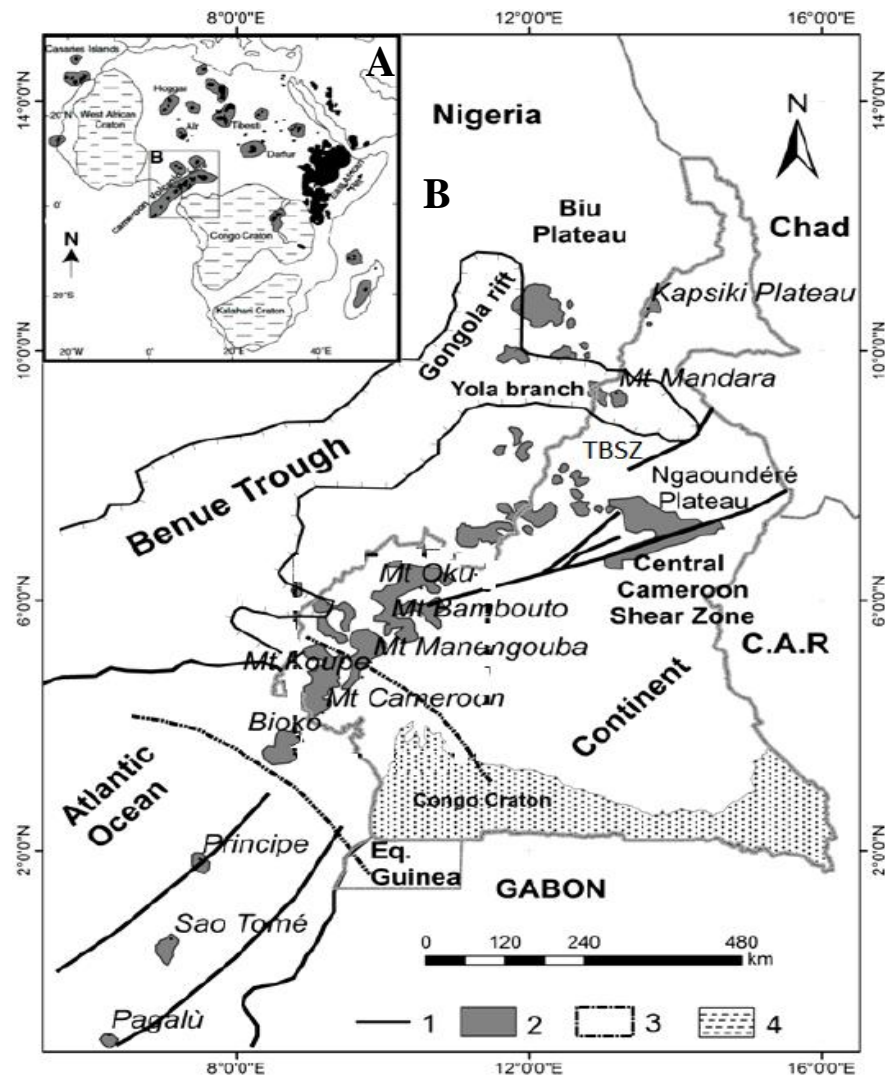
Figure 1: (A) Location map of Cameroon. (B) Simplified geological map of Cameroon and its surroundings (modified from Ngako et al. 2006). (1) Faults; (2) Cameroon volcanic line; (3) Oubanguides orogenic belt; (4) Congo Craton. TBSZ, Tchollire-Banyo shear zone.
