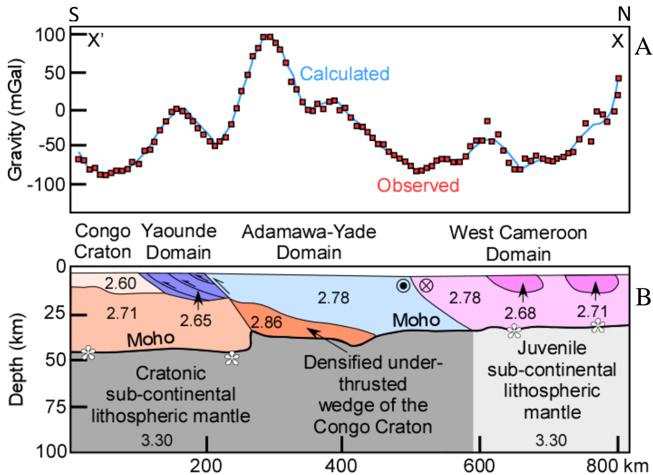
Figure 18: (A) Observed Bouguer gravity anomalies (red squares) extracted along a N-S profile flowing longitude 13°E from the World Gravity Map (WGM2012) data covering southern Cameroon and surrounding regions. Calculated Bouguer gravity anomalies are shown with a solid blue line. (B) Two-dimensional (2D) forward model illustrating the cross-sectional view of the lithospheric structure in southern Cameroon that best fit the observed Bouguer gravity anomalies of profile XX of Fig. 17. The white stars represent the Moho location of passive seismic stations of Tokam et al. (2010).
