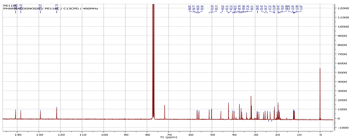
Figure 3- 23: Spectre RMN ^{13}\text{C} du composé PE.9 ( \text{CDCl}_3 , 400 MHz)
