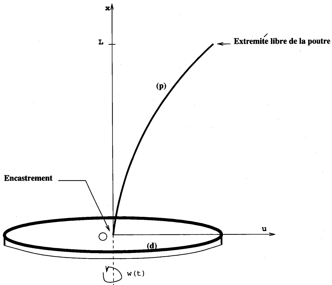
FIG. 3.1 - body-beam system
