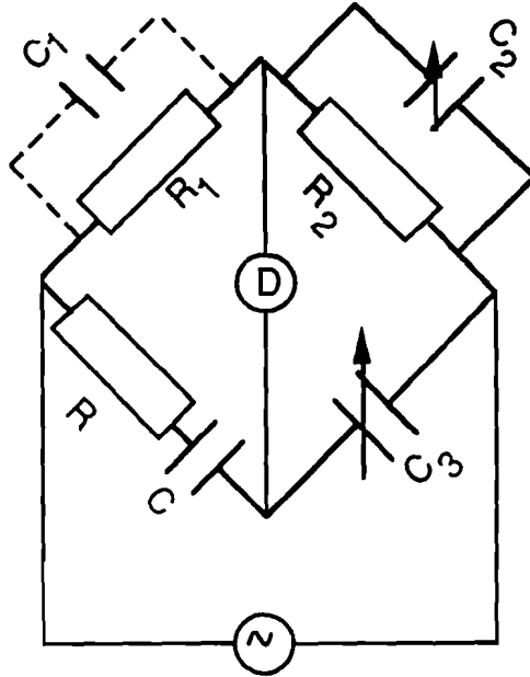
Figure 38: Pont de Schering.
