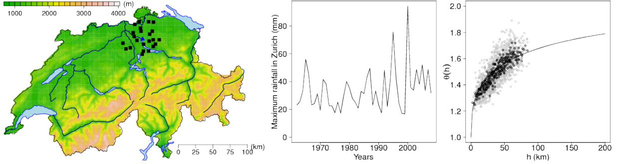
FIGURE 4.2 – Left : Map of Switzerland showing the stations of the 24 rainfall gauges used for the analysis, with an insert showing the altitude. The station marked with a triangle corresponds to Zurich. Middle : Summer maximum rainfall values for 1962–2008 at Zurich. Right : Comparison between the pairwise extremal coefficient estimates for the 51 original weather stations and the extremal coefficient function derived from a fitted Brown–Resnick processes having semi variogram \gamma(h) = (h/\lambda)^\kappa . The grey points are pairwise estimates ; the black ones are binned estimates and the curve is the fitted extremal coefficient function.
