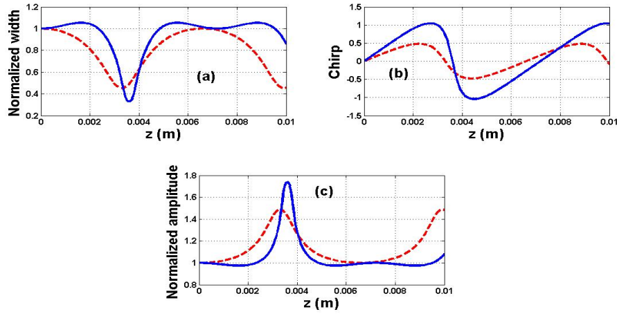
Figure 3.9: Comparison of the anomalous GVD case (red dashed curves) and the normal GVD case (blue solid curves) for the sech-type pulse : the periodic compression is enhanced in the normal GVD case. Simulation conditions are the same as in figures 3.5 and 3.8.
