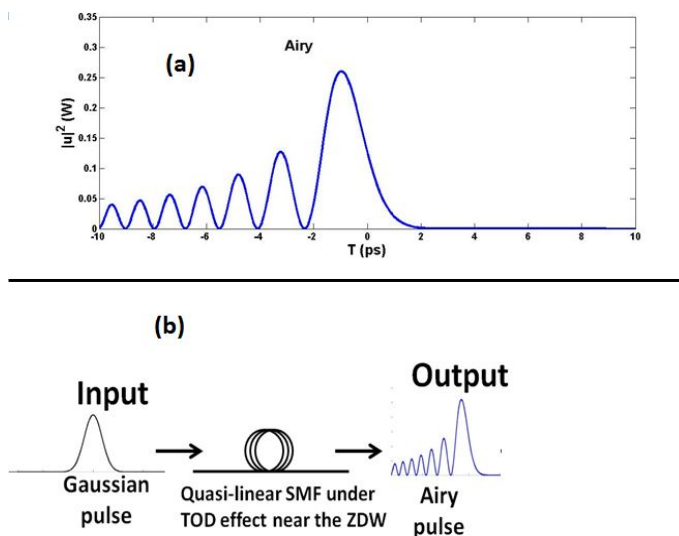
Figure 1.3: (a) Airy profile, a=0.05 , P_0 = 1 \text{ W} , r=1 , T_0 = 20 \text{ ps} ; (b) Proposed experimental set-up for obtaining an Airy pulse.
