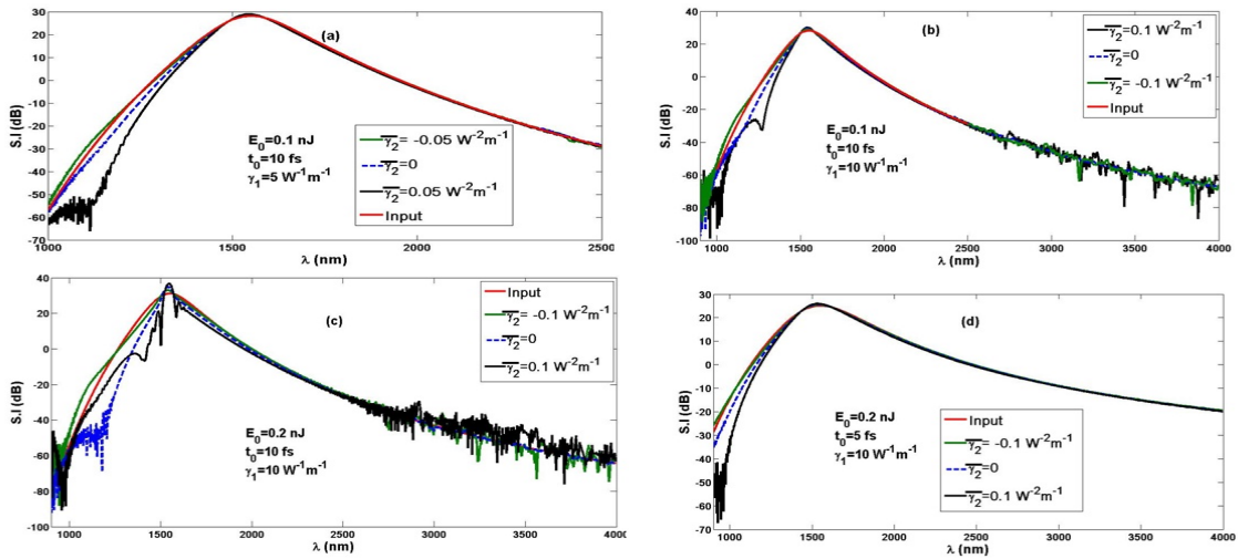
Figure 3.40: SCG spectra.
