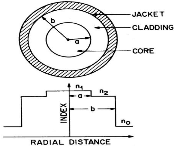
Figure 1.27: Schematic illustration of the cross section and the refractive-index profile of a step-index fiber. (©-2007 AP, from [3]).
