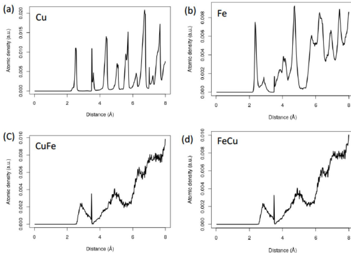
Figure 3-19. RDF of the \text{Fe}_{34}/\text{Cu}_{25}/\text{Fe}_{34} system. No considerable change is observed either for the Cu layer, FCC (a), Fe layer, BCC (b) distorted at the interface by the presence of the Cu atoms, and both interfaces remain mixed dominated by the FCC structure.
