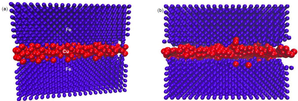
Figure 3-20 The trilayers \text{Fe}_{21}/\text{Cu}_6/\text{Fe}_{21} system before (a) and after (b) the simulated annealing. The atomic planes of Fe and Cu are shown in blue and red, respectively. One can see the presence of Fe atoms even in the bulk of the Cu layer. Additionally, the atoms of Cu disturb the structure of the Fe layer on multiple planes, thus justifying the less pronounced structure of the Fe layer close to the interface. The interfaces remain dominated by the atoms of Fe, which impose the formation of the BCC structure.
