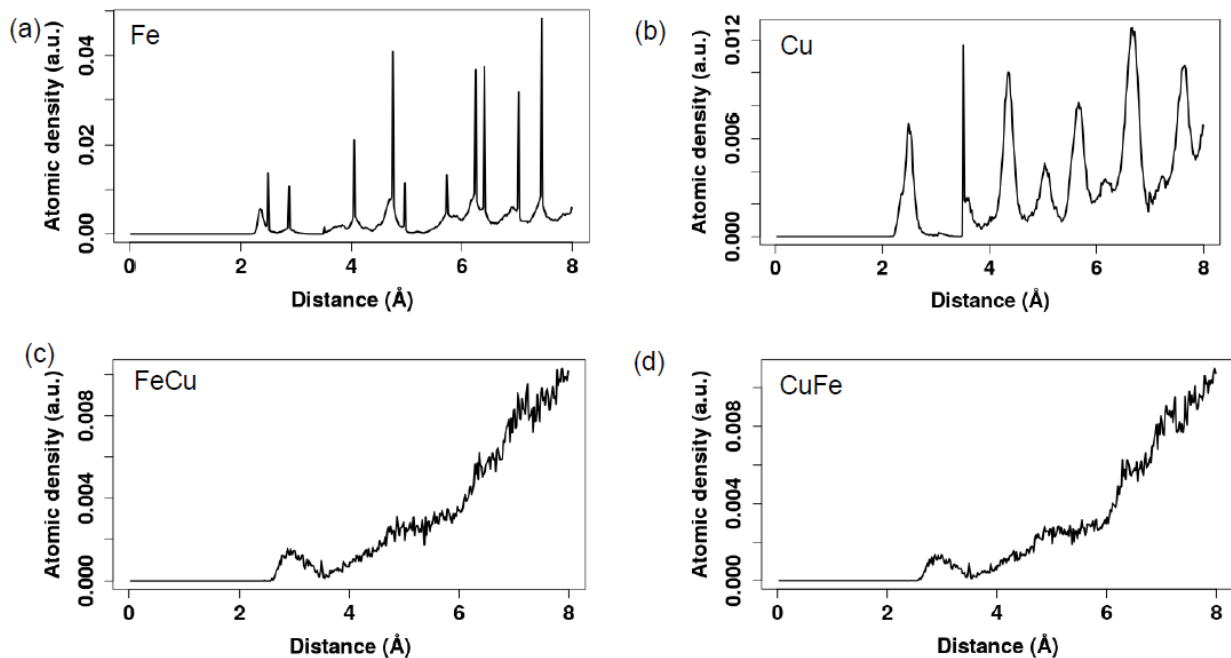
Figure 3-23. RDF of the \text{Fe}_{21}/\text{Cu}_{13}/\text{Fe}_{21} system. Fe has conserved its BCC structure, less disturbed by the presence of the Cu atoms (a). During the growth process, atoms of Cu will tend to form an agglomerates composed uniquely of Cu atoms, thus limiting the disturbance of the Fe layer at the interface. (b) shows the FCC structure of Cu, while the effect of the transition is seen at the interface (c, d).
