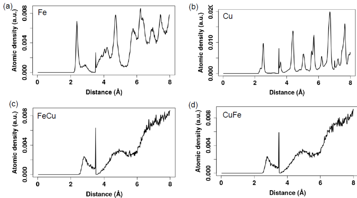
Figure 3-25. RDF of Fe 21 /Cu 24 /Fe 21 system. The disturbance is again seen at the interface of the Fe layer (a), which is still BCC, as the thickness of the Cu continues to grow. (b) shows the FCC structure of the Cu layer. In the presence of a high atomic proportion of Cu at the interface, Fe atoms will tend to copy the FCC structure of the interface (c, d) for the first atomic planes. This can justify the mixed structure dominated by the FCC of the interface.
